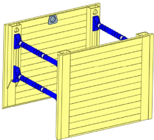
Grundelement H= 2,0 m
